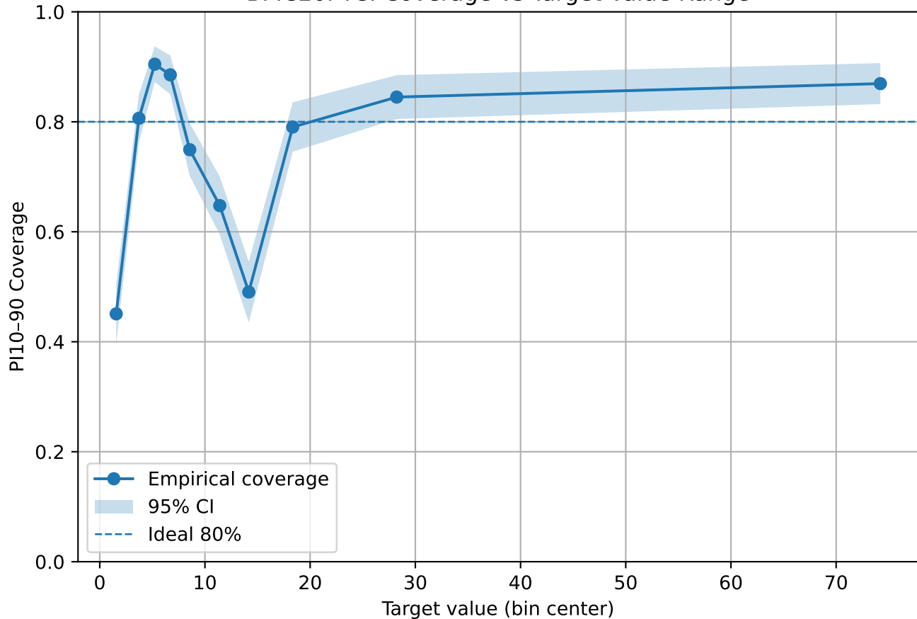
BPIC20PTC: Coverage vs Target Value Range
